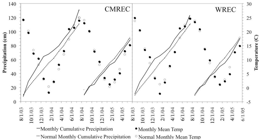
Fig. 2. Mean monthly temperature and cumulative monthly precipitation at University of Maryland Central Maryland Research and Education Center-Beltsville facility (CMREC) and Wye Research and Education Center (WREC) from 1 Aug. 2003 through 31 May 2005. The normal data are based on 30-yr averages at each site. Precipitation data are cumulative from 1 Aug. 2003 to 31 July 2004 and from 1 Aug. 2004 to 31 May 2005.
