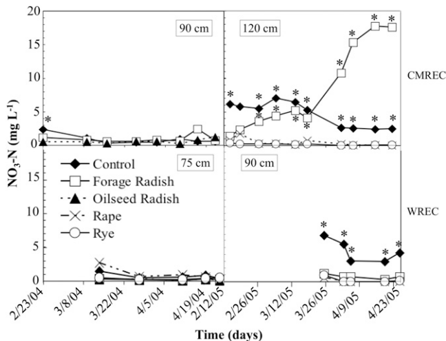
Fig. 5. Soil pore water nitrate-nitrogen at University of Maryland Central Maryland Research and Education Center-Beltsville facility (CMREC) and Wye Research and Education Center (WREC) in the spring of 2004 and 2005. Means from four lysimeters per treatment in spring 2004 and eight lysimeters per treatment (two per plot, four plots sampled) in spring 2005 are shown. Lysimeters were sampled weekly. Depth of lysimeter placement was 90 and 120 cm at CMREC and 75 and 90 cm at WREC in spring 2004 and 2005, respectively. *Significantly greater means than smallest mean for each date sampled ( p < 0.1 ).
