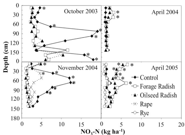
Fig. 3. Soil nitrate-nitrogen amounts for each 15-cm depth increment sampled at University of Maryland Central Maryland Research and Education Center-Beltsville facility from October 2003 through April 2005. *Significantly greater means than smallest mean within a depth increment ( p < 0.1 ).
