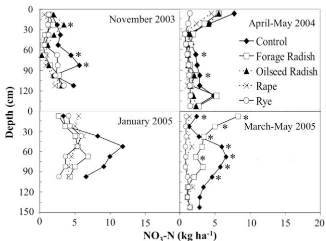
Fig. 4. Soil nitrate-nitrogen for each 15-cm depth increment sampled at Univ. of Maryland Wye Research and Education Center from November 2003 through May 2005. *Significantly greater means than smallest mean within a depth increment ( p < 0.1 ).
